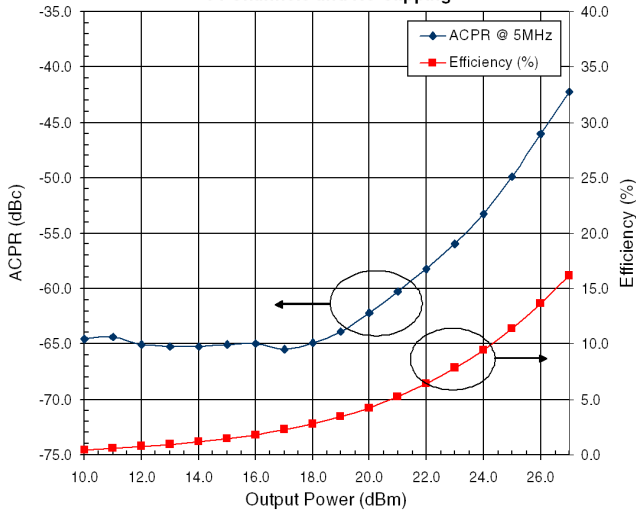
3809411 @ 882 MHz W-CDMA 64 Channels and No Clipping
