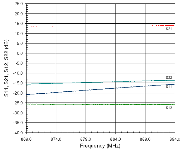
RF3809413 Evaluation Board S-Parameters
