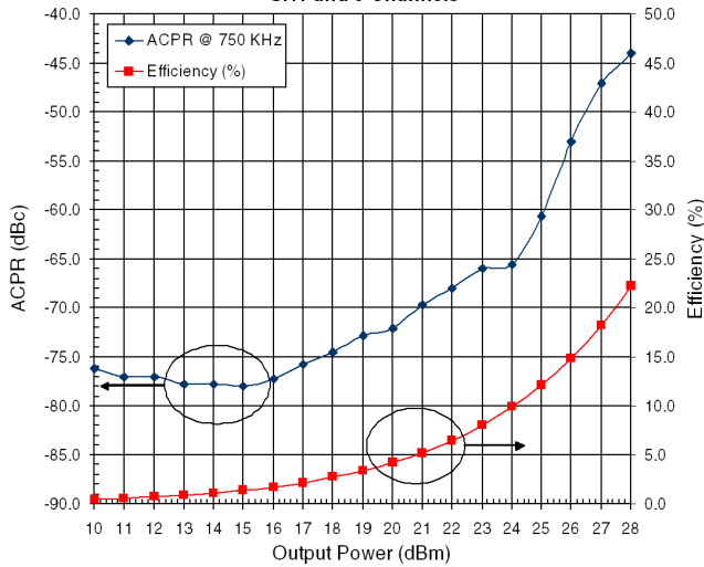
RF3809414 @ 1960 MHz CDMA2K SR1 and 9 Channels
