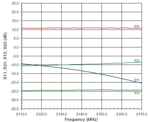
RF3809415 Evaluation Board S-Parameters
