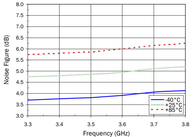
Noise Figure (NF) versus Frequency
