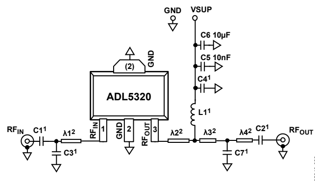
Figure 26. Basic Connections
