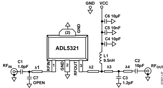
Figure 30. Evaluation Board, 2500 MHz to 2700 MHz
