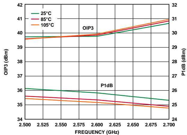
Figure 28. OIP3 and P1dB vs. Frequency and Temperature, 2.5 GHz to 2.7 GHz
