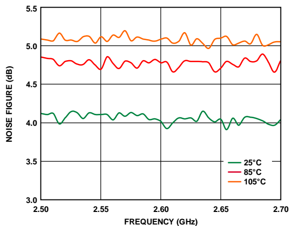
Figure 29. Noise Figure vs. Frequency and Temperature, 2.5 GHz to 2.7 GHz
