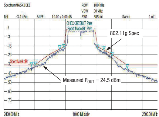
Spectral Response (802.11g 64 QAM @ 54 Mbps Input Signal)
