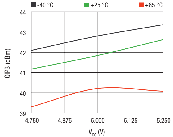
OIP3 vs. V_{CC} Across Temperature, P_{IN}/\text{Tone} = -2\text{ dBm}
