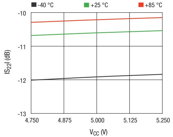
|S 22 | vs. V CC Across Temperature
