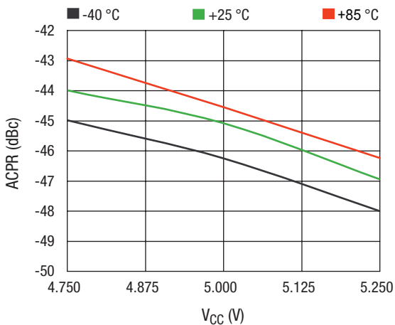
ACPR vs. V CC Across Temperature @ P OUT = 19 dBm
