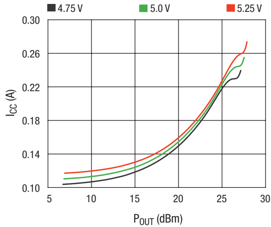
I CC vs. P OUT Across Voltage
