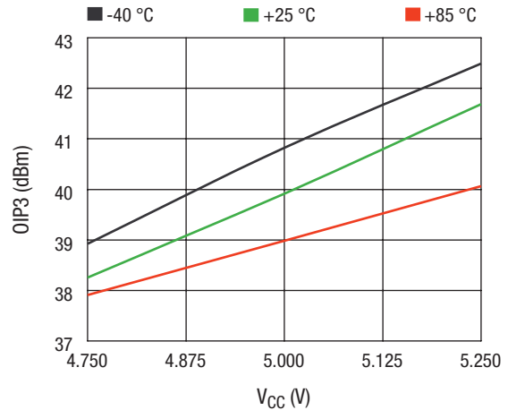
OIP3 vs. V_{CC} Across Temperature, P_{1M}/\text{Tone} = 0\text{ dBm}
