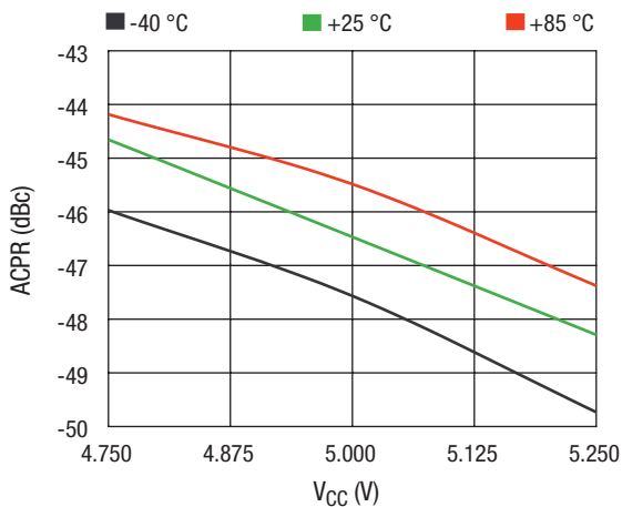
ACPR vs. V CC Across Temperature @ P OUT = 20 dBm
