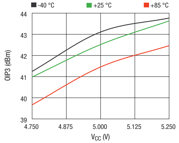
OIP3 vs. V_{CC} Across Temperature, P_{IN}/\text{Tone} = 0\text{ dBm}
