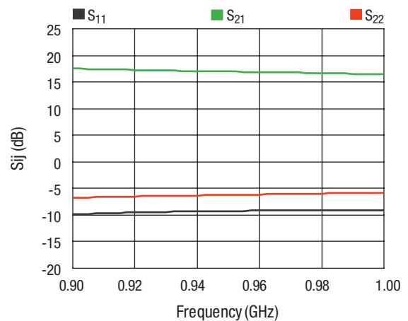
SP vs. Frequency T = 25 °C Tuned for 900 MHz
