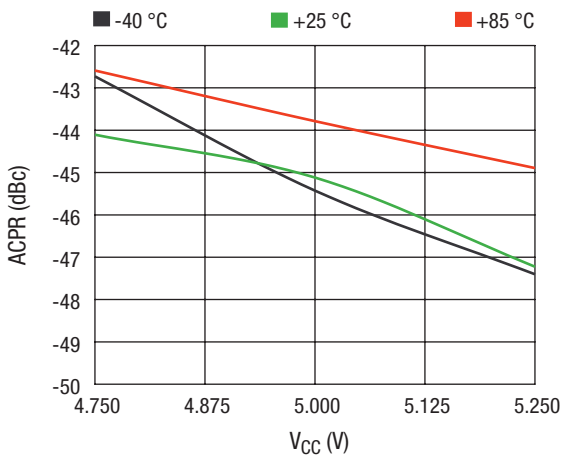
ACPR vs. V CC Across Temperature @ P OUT = 18 dBm
