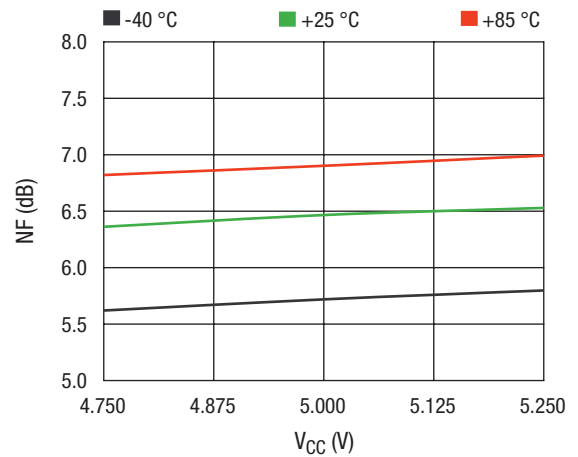
NF vs. V CC Across Temperature
