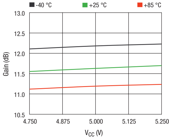
Gain vs. V_{CC} Across Temperature @ P_{IN} -15\ \text{dBm}
