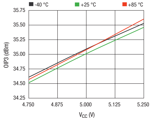
OIP3 vs. V CC Across Temperature, P IN /Tone = -5 dBm
