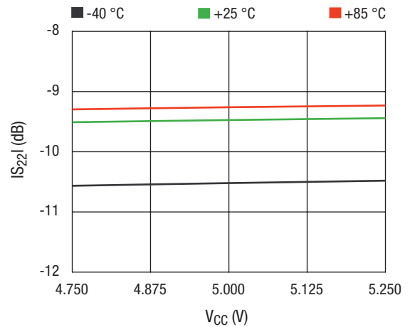
|S 22 | vs. V CC Across Temperature
