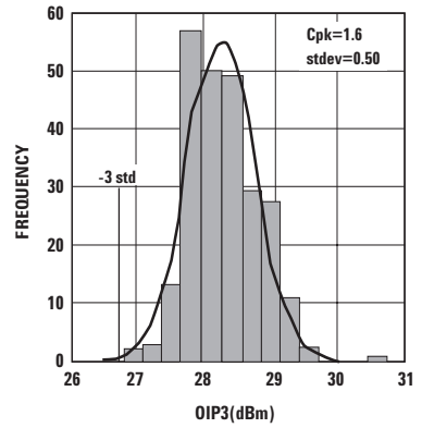
Figure 4. OIP3 @ 2 GHz 3V 40 mA. LSL=26, Nominal=28.5.
