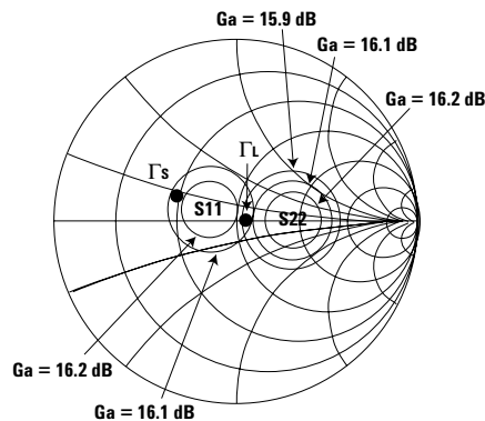
Figure 18. Input and output gain circles.
