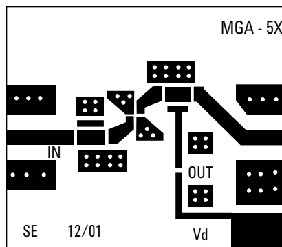
Figure 16. MGA-53543 PCB Layout.
