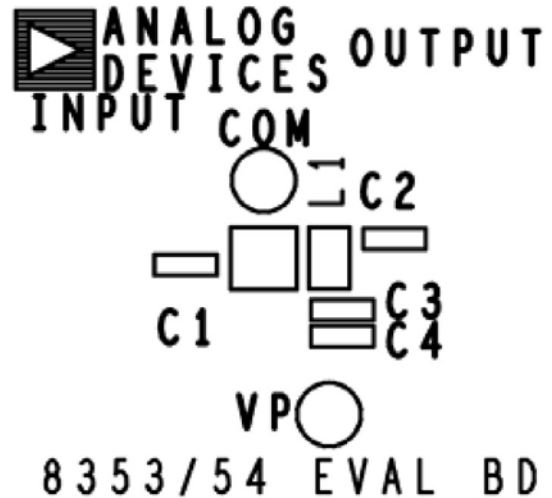
Figure 41. Silkscreen Top
