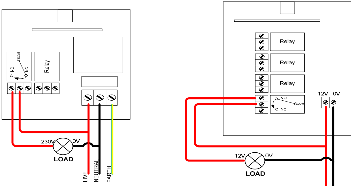
HORNET 230V Systems 230V Switched Output Example— Only to be used by a competent person
