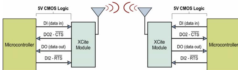
Figure 2-01. Data Flow in a UART-interfaced environment
