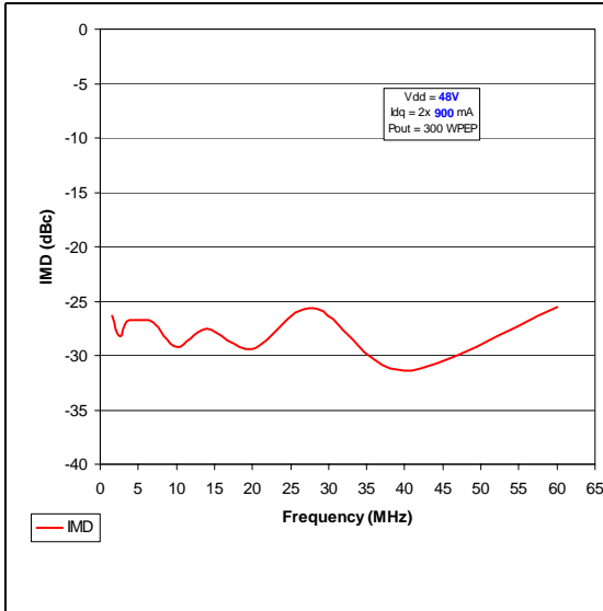
Figure 3. IMD vs. frequency
