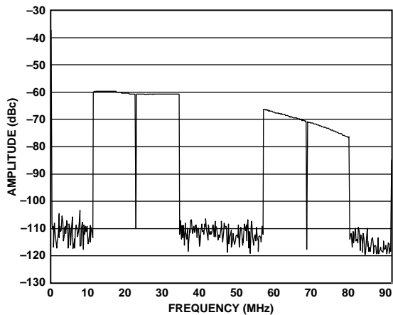
Figure 66. AD9861 Tx Path FFT of OFDM Signal in Figure 52 with 1x Interpolation
