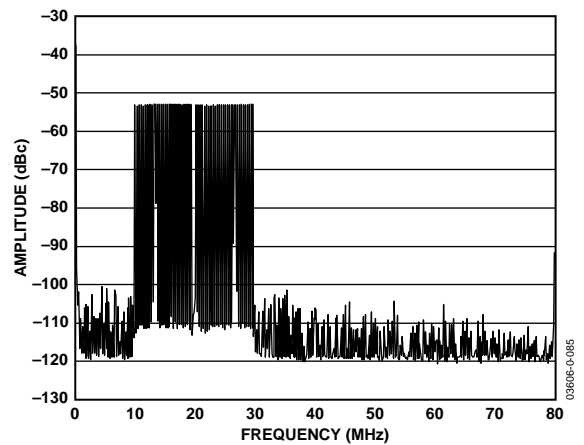
Figure 57. AD9861 Tx Path FFT of OFDM Signal in Figure 52, with 4x Interpolation
