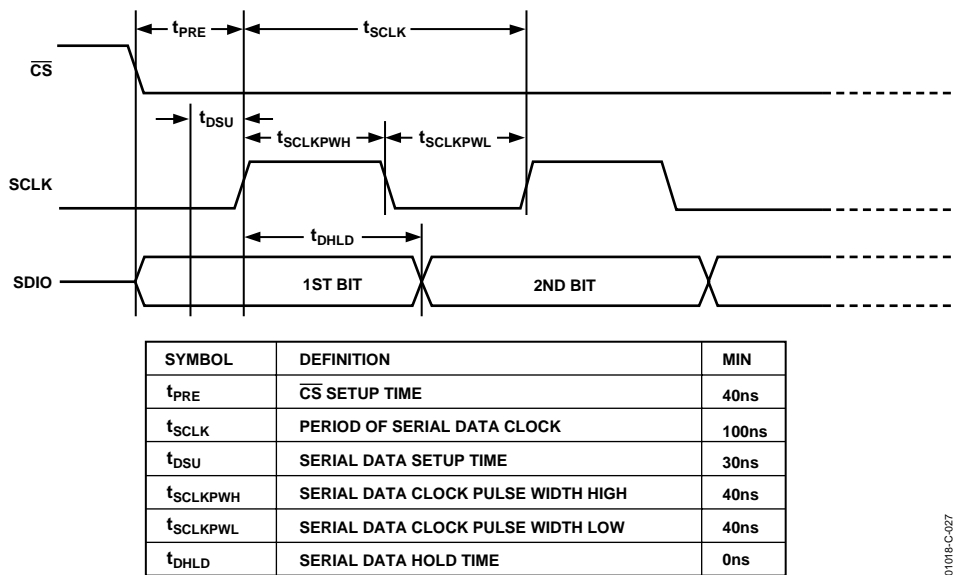
Figure 27. Timing Diagram for Data Write to AD9857
