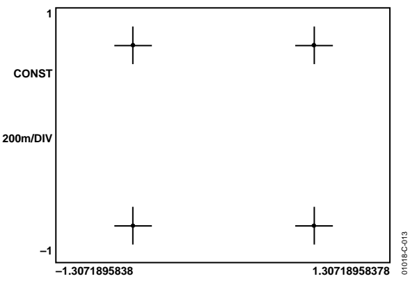
Figure 13. QPSK, 65 MHz, 2.56 MS/s
