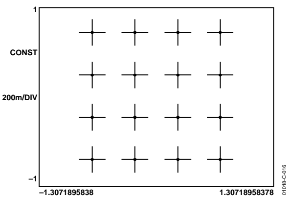
Figure 16. 16-QAM, 65 MHz, 2.56 MS/s
