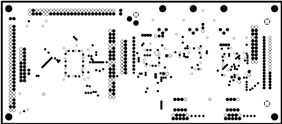
GROUND PLANE LAYERS 3 & 6 (CB6624CE.pho)
