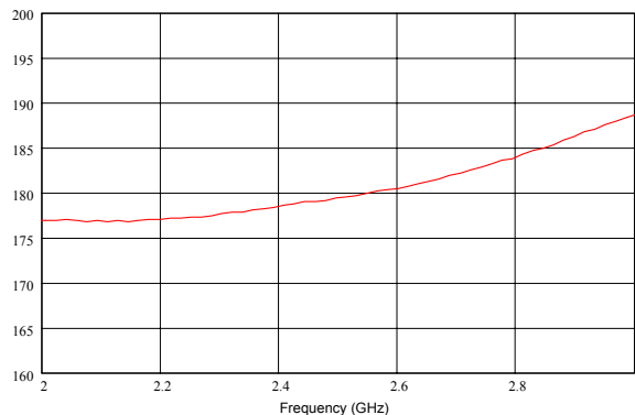
Phase Balance (degree)
