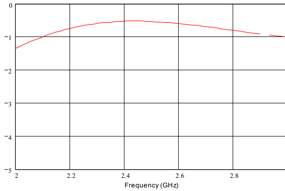
Insertion Loss (dB)
