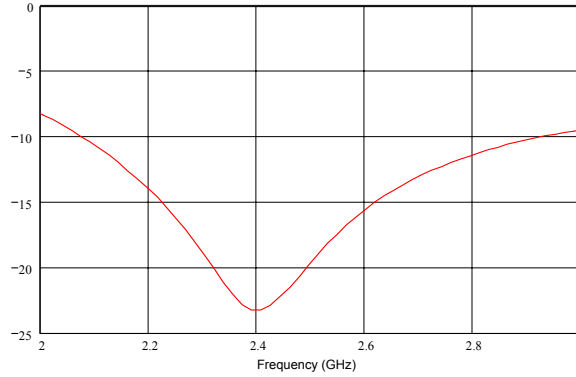
Return Loss (dB)
