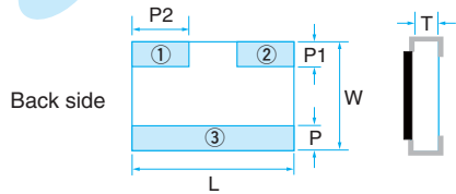
RAT1010X, PAT1220, PAT1632, PAT3042S
