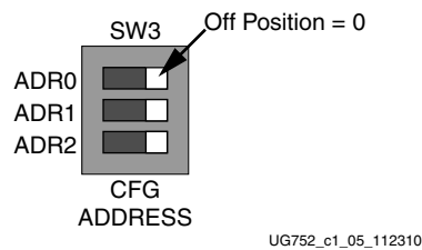
Figure 1-5: DIP Switch SW3 Settings For Duals 101 and 123
