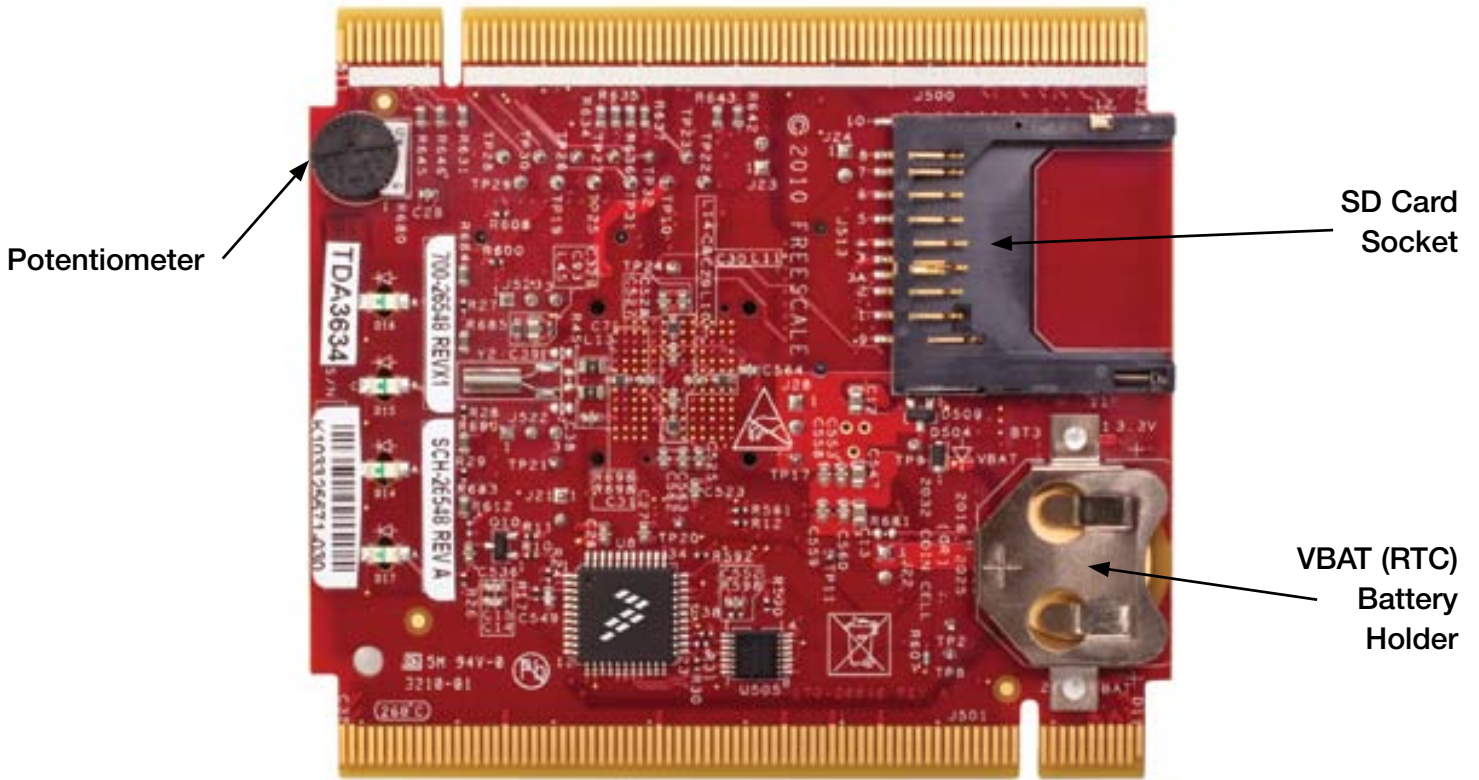
Figure 2: Back Side of TWR-K60N512 Module.
