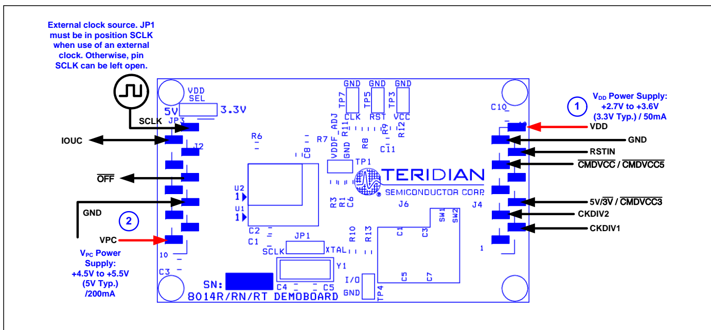
Figure 2: 73S8014R/RN/RT Demo Board: Basic Connections
