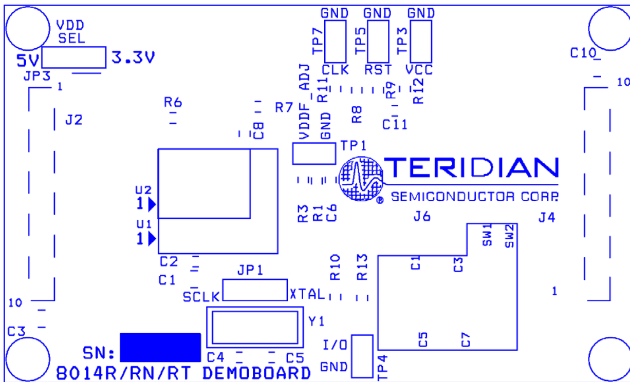
Figure 5: TERIDIAN 73S8014R/RN/RT 20SO Demo Board: Top View
