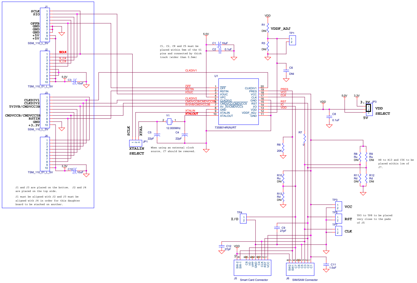
Figure 4: TERIDIAN 73S8014R/RN/RT 20SO Demo Board: Electrical Schematic
