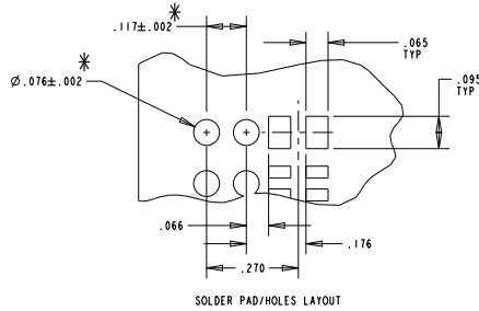
SOLDER PAD/HOLES LAYOUT
