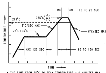
* THE TIME FROM 25°C TO PEAK TEMPERATURE = 6 MINUTES MAX RECOMMENDED RoHS SOLDER PROFILE
