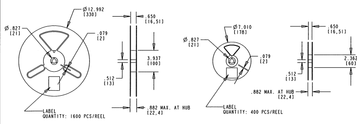
13 INCH DIA. REEL SPECIFICATIONS
