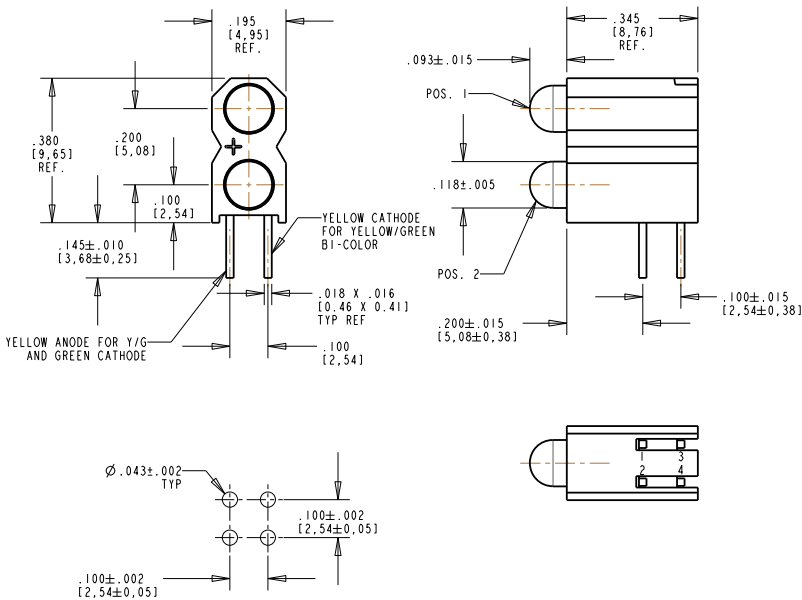
RECOMMENDED HOLE PATTERN GAUGE
