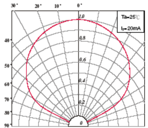
Radiation pattern
