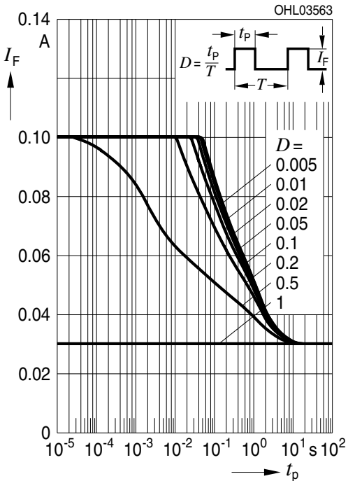
Zulässige Impulsbelastbarkeit Permissible Pulse Handling Capability Duty cycle D = \text{parameter} , T_S = 85\text{ °C} I_F = f(t_p) ; red (1 Chip on)
