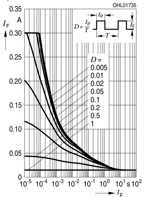
Zulässige Impulsbelastbarkeit Permissible Pulse Handling Capability Duty cycle D = \text{parameter} , T_S = 85\text{ °C} I_F = f(t_p) ; blue (3 Chips on)
