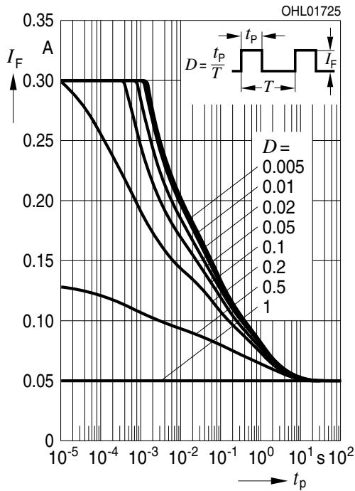
Zulässige Impulsbelastbarkeit Permissible Pulse Handling Capability Duty cycle D = \text{parameter} , T_S = 85\text{ °C} I_F = f(t_p) ; blue (1 Chip on)
