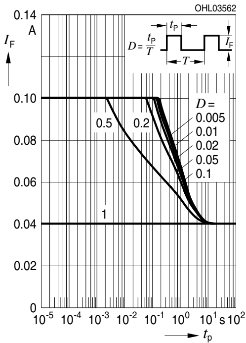
Zulässige Impulsbelastbarkeit Permissible Pulse Handling Capability Duty cycle D = \text{parameter} , T_S = 85\text{ °C} I_F = f(t_p) ; red (1 Chip on)
