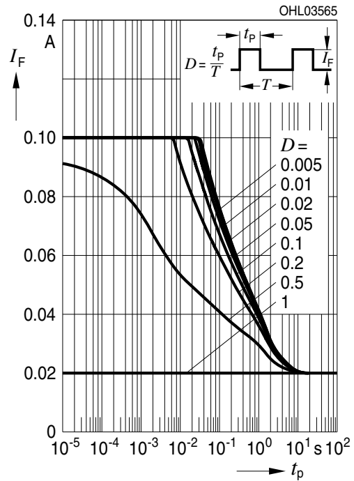
Zulässige Impulsbelastbarkeit Permissible Pulse Handling Capability Duty cycle D = \text{parameter} , T_S = 85\text{ °C} I_F = f(t_p) ; red (3 Chips on)
