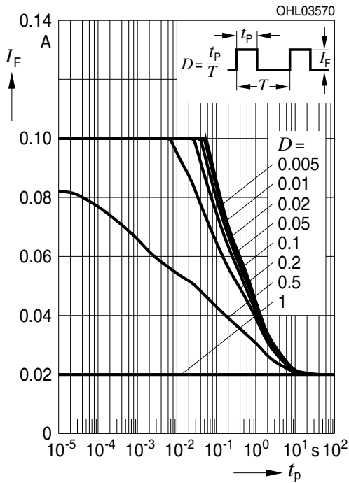
Zulässige Impulsbelastbarkeit Permissible Pulse Handling Capability Duty cycle D = \text{parameter} , T_A = 85^\circ\text{C} I_F = f(t_p) ; true green (1 Chip on)
