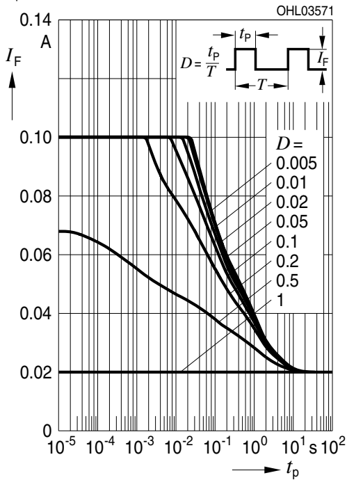
Zulässige Impulsbelastbarkeit Permissible Pulse Handling Capability Duty cycle D = \text{parameter} , T_A = 85^\circ\text{C} I_F = f(t_p) ; true green (1 Chip on)
