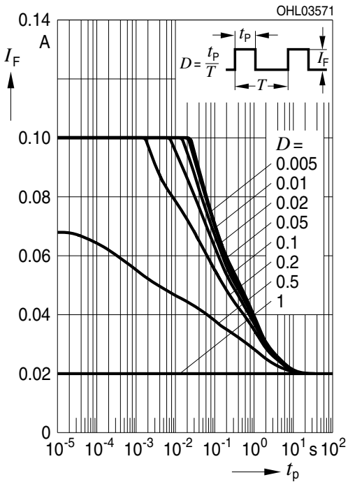
Zulässige Impulsbelastbarkeit Permissible Pulse Handling Capability Duty cycle D = parameter, T_A = 85\text{ °C} I_F = f(t_p) ; blue (1 Chip on)
