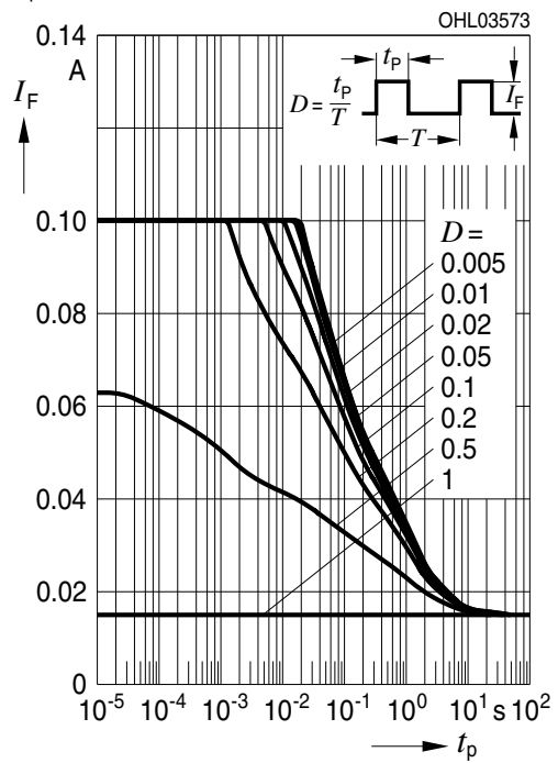
Zulässige Impulsbelastbarkeit Permissible Pulse Handling Capability Duty cycle D = \text{parameter} , T_A = 85^\circ\text{C} I_F = f(t_p) ; true green (3 Chips on)
