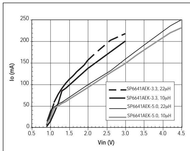
Figure 13. SP6641AEK-3.3 & SP6641AEK-5.0 Maximum Resistive Load Current in Startup
