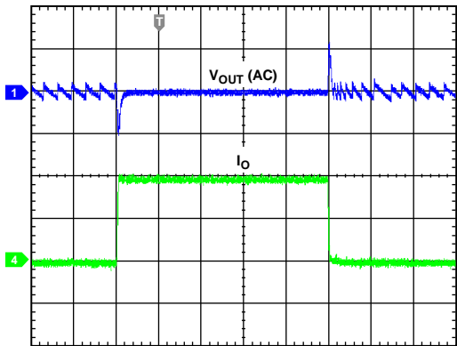
Figure 23. Load Transient (ADP2119, PFM, V_{IN} = 5V )
