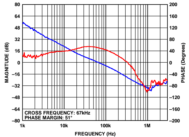
Figure 45. ADP2120 Bode Plot at V_{IN} = 5\text{ V} , V_{OUT} = 1.5\text{ V} , I_O = 1.25\text{ A} , L = 2.2\ \mu\text{H} , C_{OUT} = 22\ \mu\text{F} + 10\ \mu\text{F}
