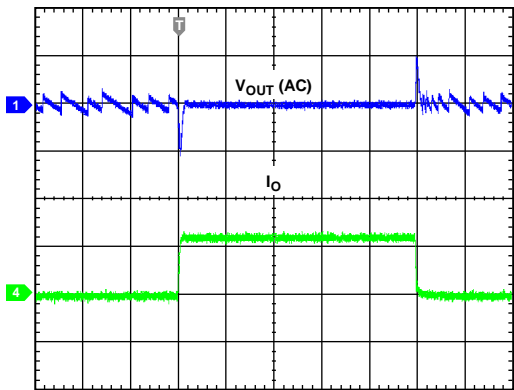
Figure 24. Load Transient (ADP2120, PFM, V_{IN} = 5V )
