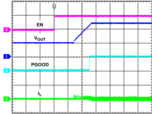
Figure 25. Soft Start with Precharged Output (ADP2119, V_{IN} = 5V )
