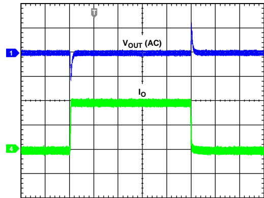
Figure 26. Load Transient (ADP2119, FPWM, V_{IN} = 5V )
