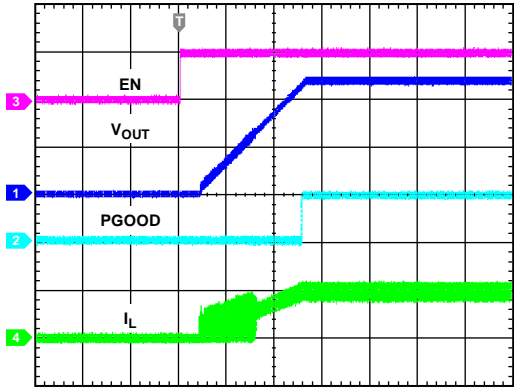
Figure 22. Soft Start with Full Load (ADP2119, V_{IN} = 5V )
