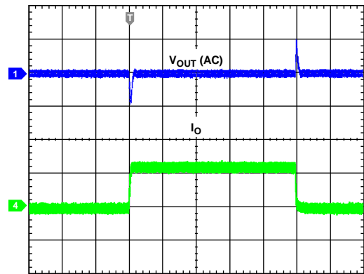
Figure 27. Load Transient (ADP2120, FPWM, V_{IN} = 5V )
