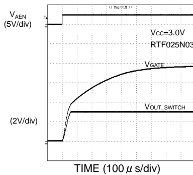
Fig.26 GATE Switch Rise Characteristics
