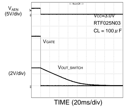
Fig.28 GATE Switch Fall Characteristics
