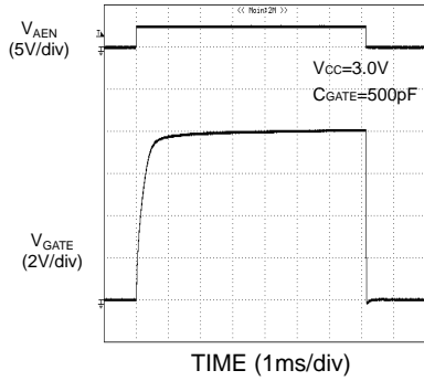
Fig.23 GATE Rise / Fall Characteristics
