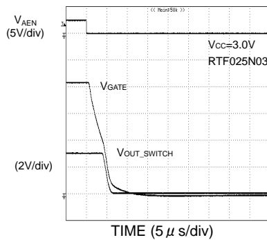
Fig.27 GATE Switch Fall Characteristics
