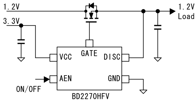
Fig.37 Configuration of Low-voltage Load Switch
