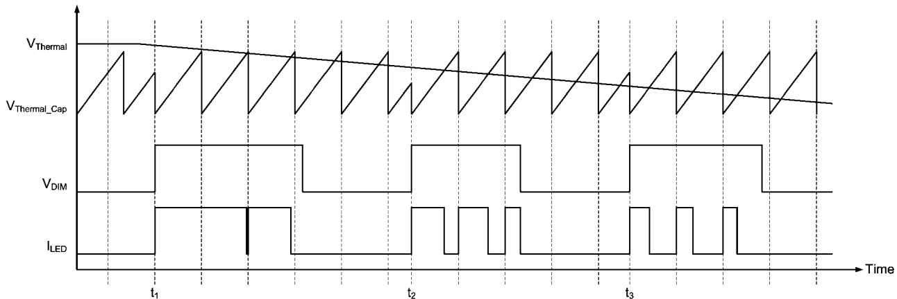
FIGURE 11. Thermal Foldback + PWM Dimming Control
