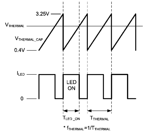
FIGURE 9. Signals Facilitating Thermal Foldback Control
