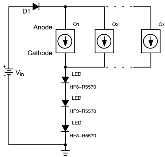
Figure 8. Typical Application Circuit (30 mA each LED String)
