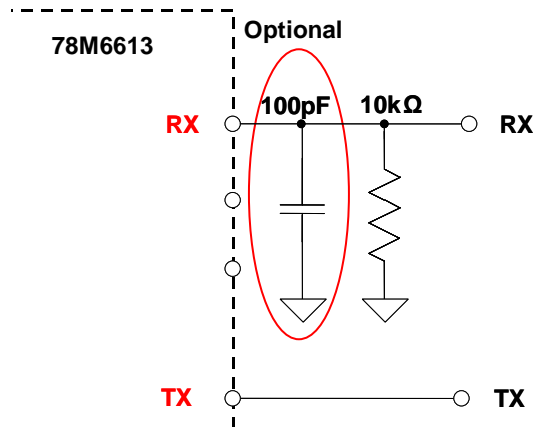
Figure 10: Connections for the RX Pin
