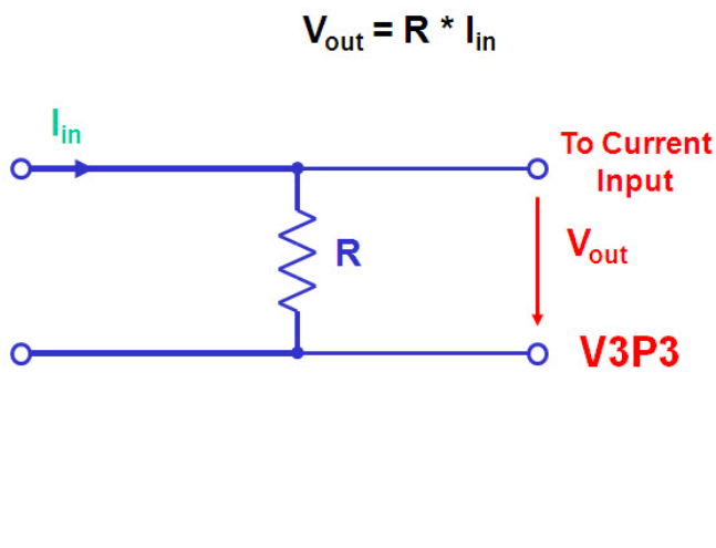
Figure 8: Resistive Current Shunt
