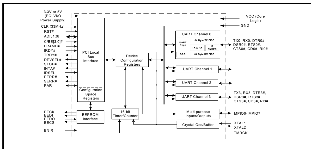
FIGURE 1. BLOCK DIAGRAM
