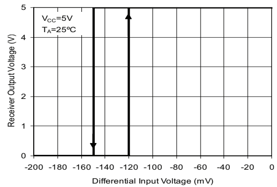
Receiver Output Voltage vs Differential Input Voltage
