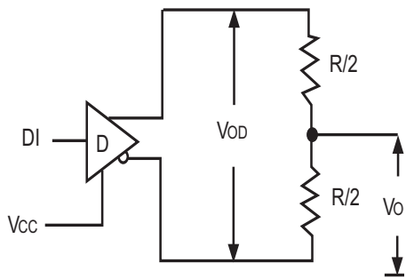
Driver DC Test Circuit
