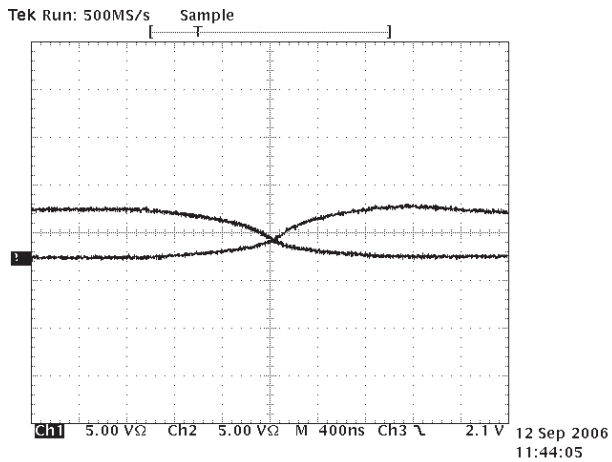
Driver output Waveform High to Low (SP3080-SP3082)
