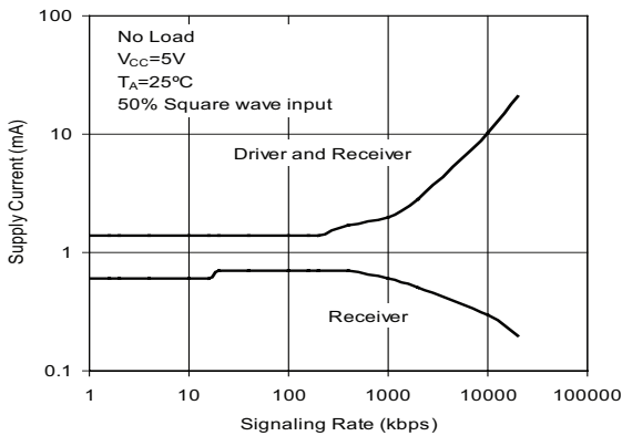
Supply Current vs Signaling Rate (SP3086-SP3088)
