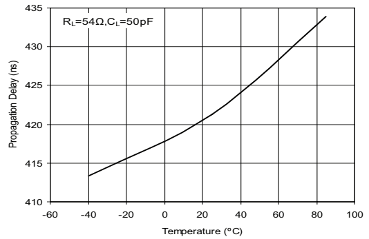
Driver Average Propagation Delay vs Temperature (SP3083-SP3085)
