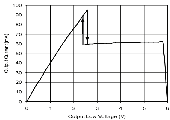
Output Current vs Driver Output Low Voltage
