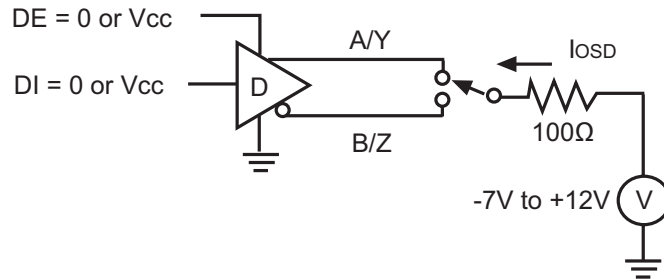
Driver Short Circuit Current Limit Test Circuit
