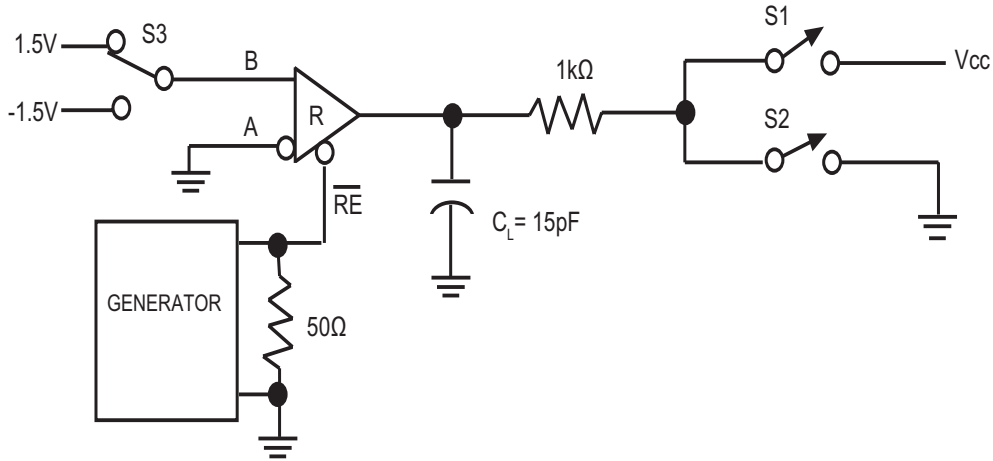
Receiver Enable and Disable Timing Diagram
