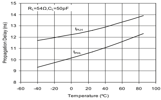
Driver Propagation Delay vs Temperature (SP3086-SP3088)
