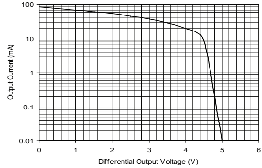
Driver Output Current vs Differential Output Voltage
