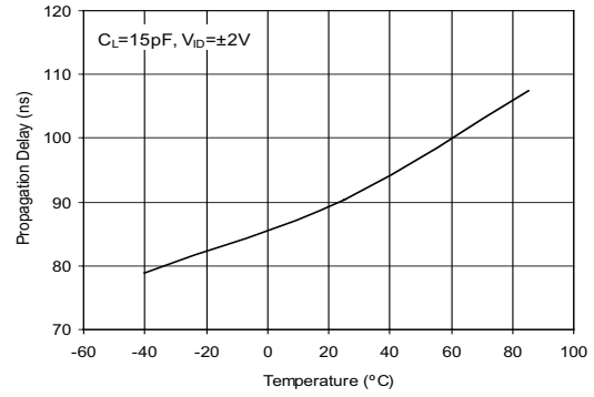
Receiver Average Propagation Delay vs Temperature (SP3080-SP3082)
