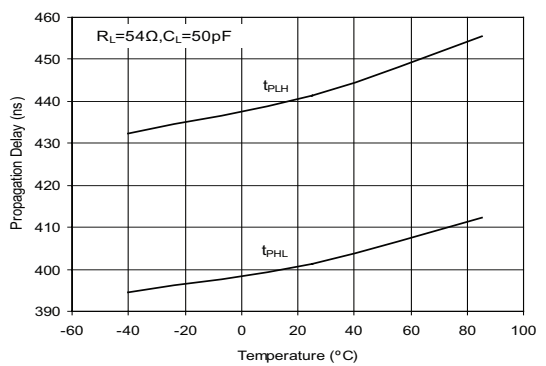
Driver Propagation Delay vs Temperature (SP3083-SP3085)
