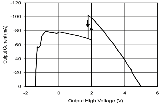
Output Current vs Driver Output High Voltage
