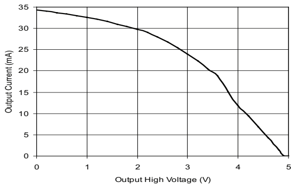
Output Current vs Receiver Output High Voltage
