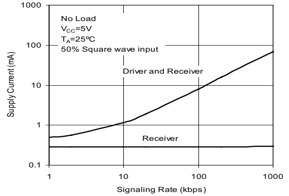
Supply Current vs Signaling Rate (SP3083 - SP3085)
