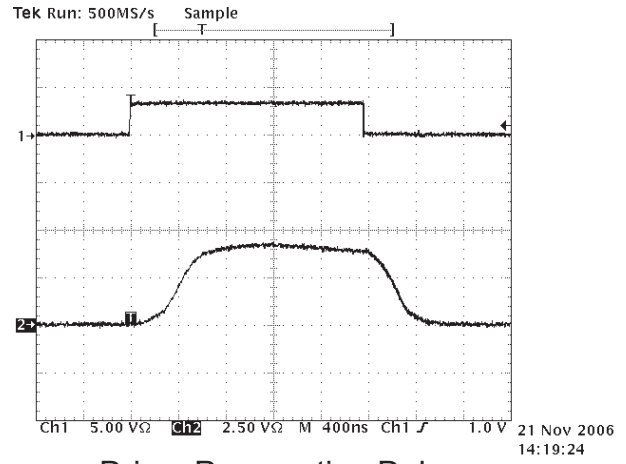
Driver Propagation Delay (SP3083-SP3085)
