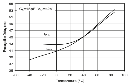
Receiver Propagation Delay vs Temperature (SP3086-SP3088)
