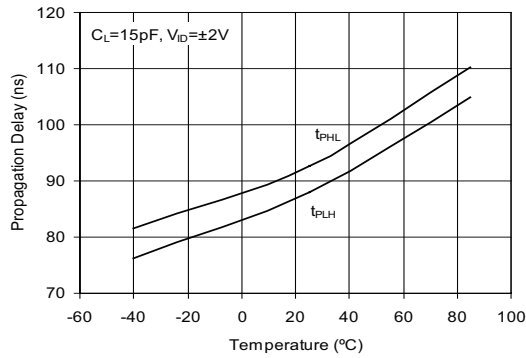
Receiver Propagation Delay vs Temperature (SP3080-SP3082)
