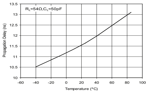
Driver Average Propagation Delay vs Temperature (SP3086-SP3088)
