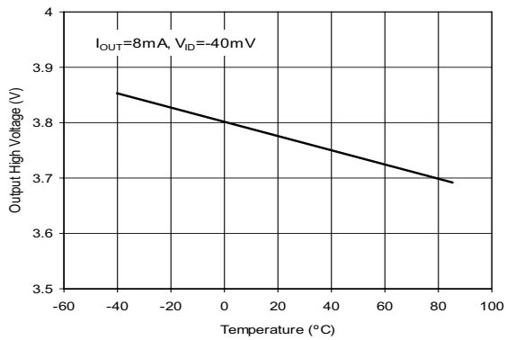
Receiver Output High Voltage vs Temperature
