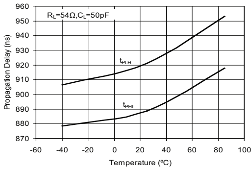
Driver Propagation Delay vs Temperature (SP3080-SP3082)
