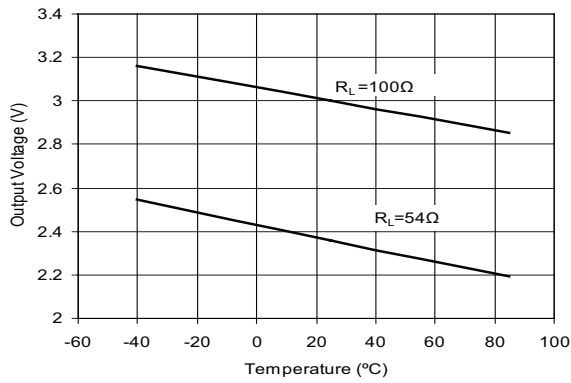
Driver Differential Output Voltage vs Temperature
