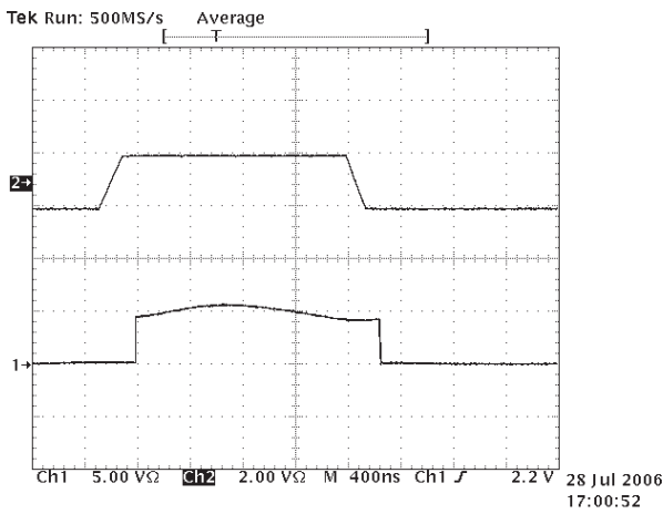
Receiver Propagation Delay (SP3083-SP3085)
