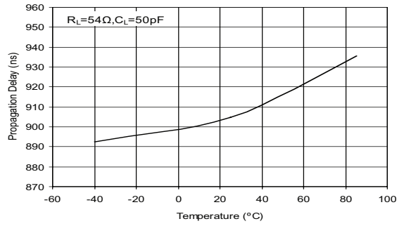
Driver Average Propagation Delay vs Temperature (SP3080-SP3082)
