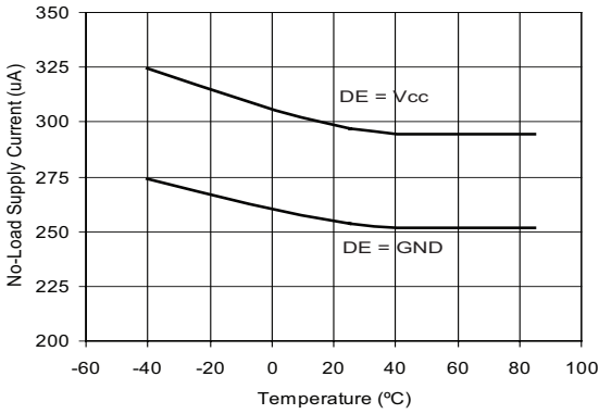
No-Load Supply Current vs Temperature
