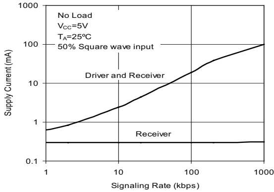
Supply Current vs Signaling Rate (SP3080-SP3082)
