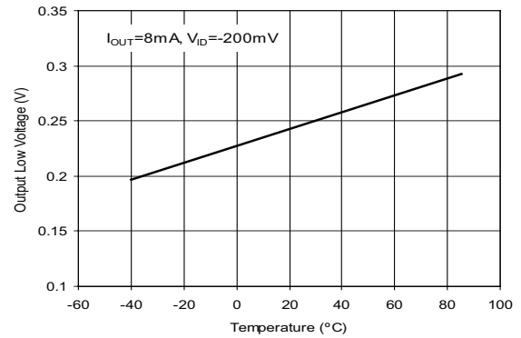
Receiver Output Low Voltage vs Temperature
