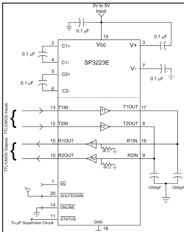
Figure 14. Loopback Test Circuit for RS-232 Driver
