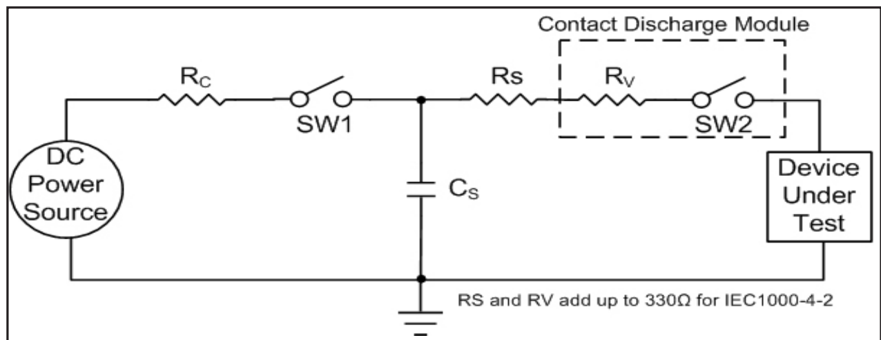
Figure 25. ESD Test Circuit for IEC1000-4-2
