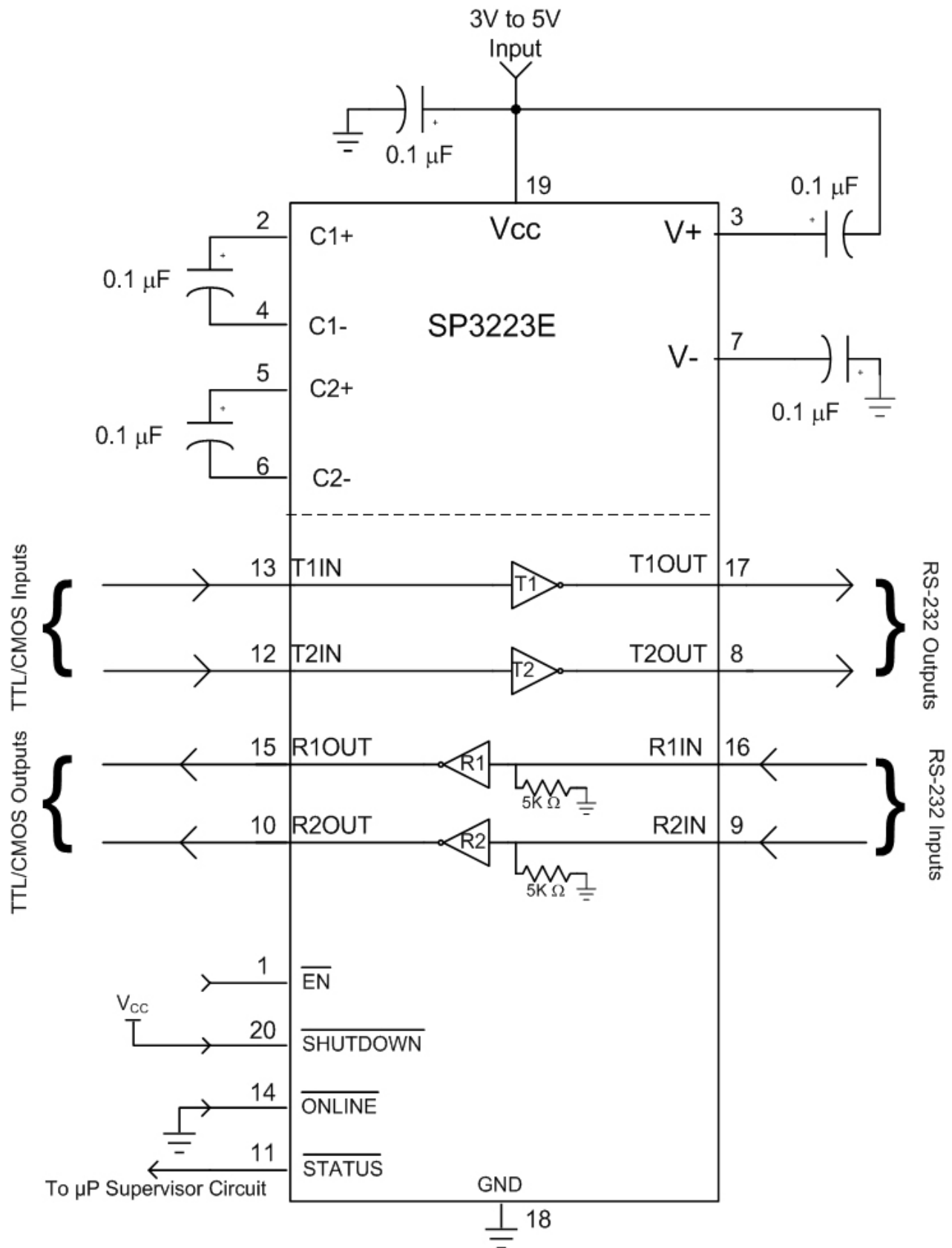
Figure 1. SP3223E Typical Operating Circuit
