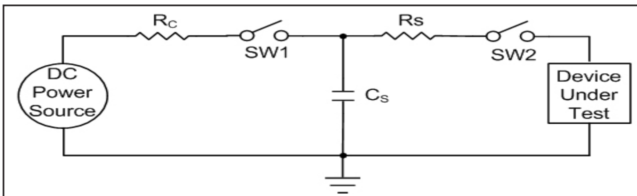
Figure 24. ESD Test Circuit for Human Body Model
