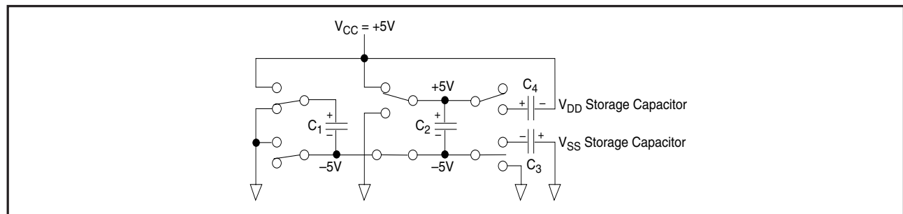
Figure 20. Charge Pump - Phase 3
