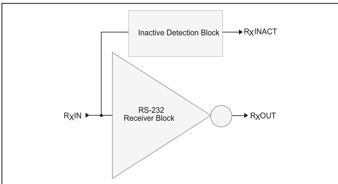
Figure 22. Stage I of AUTO ON-LINE® Circuitry
