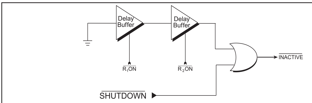
Figure 23. Stage II of AUTO ON-LINE® Circuitry
