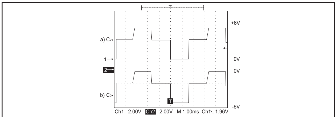
Figure 19. Charge Pump Waveforms
