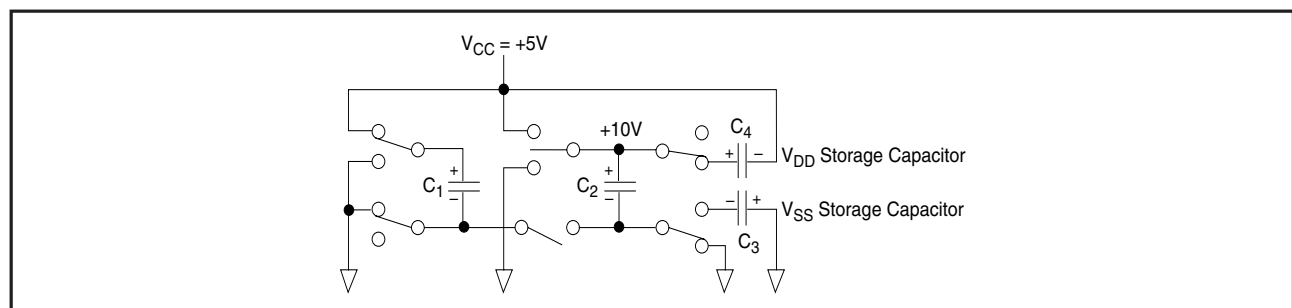
Figure 21. Charge Pump - Phase 4
