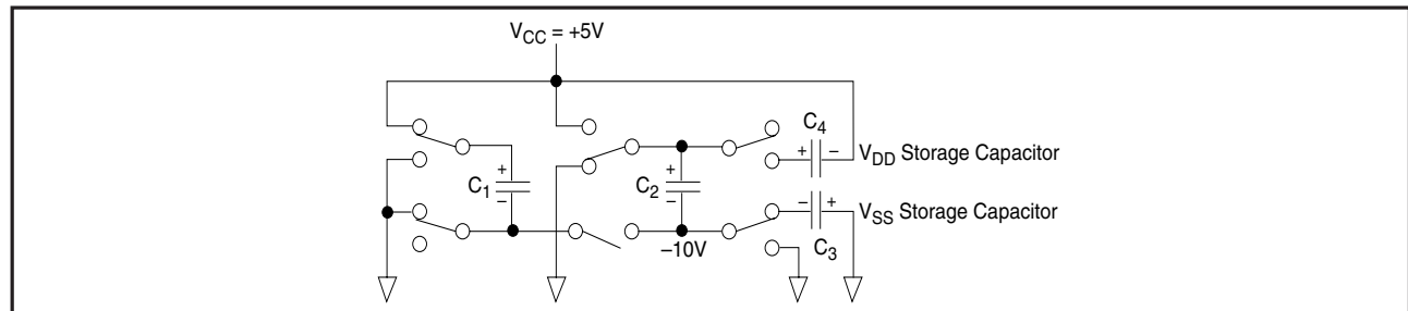
Figure 18. Charge Pump - Phase 2
