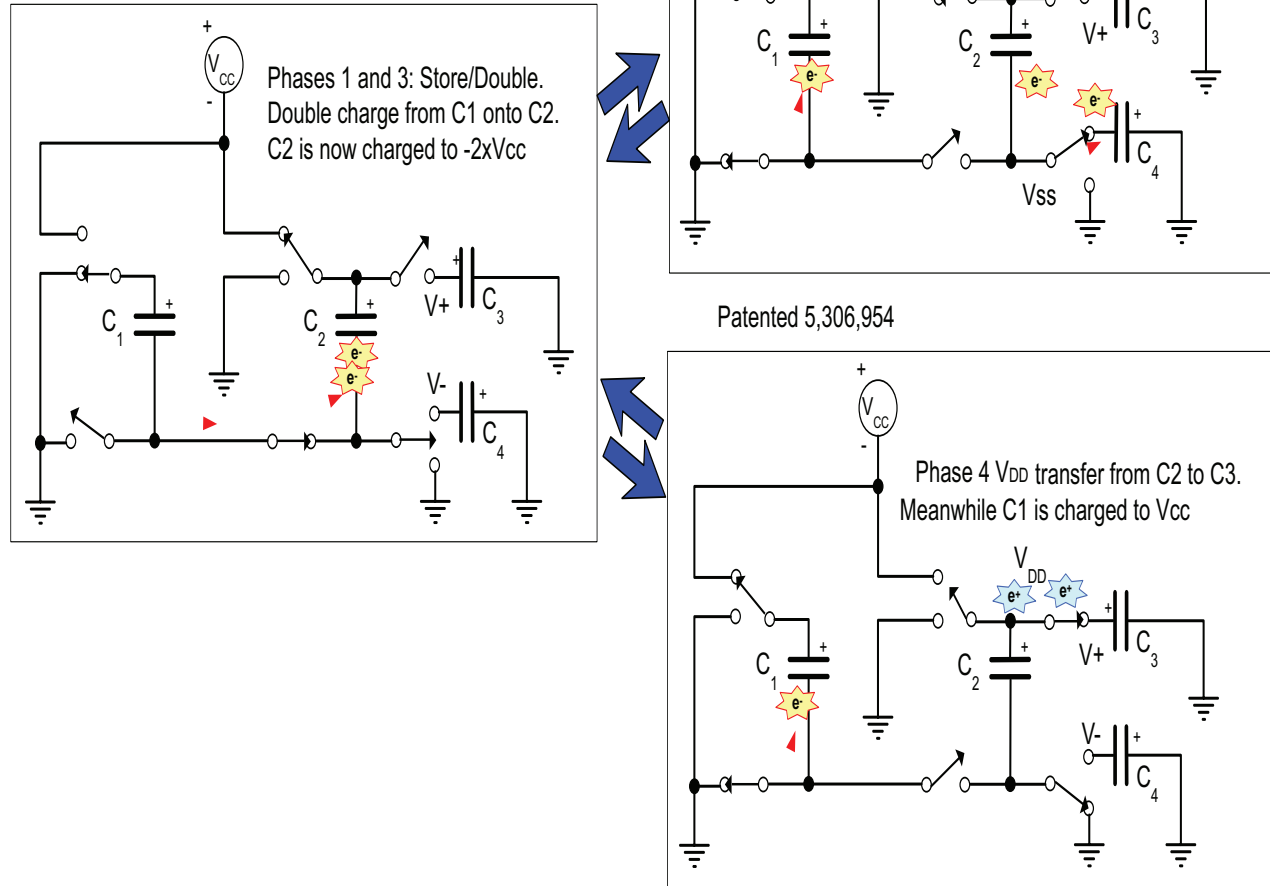
Figure 1. Charge pump phases
