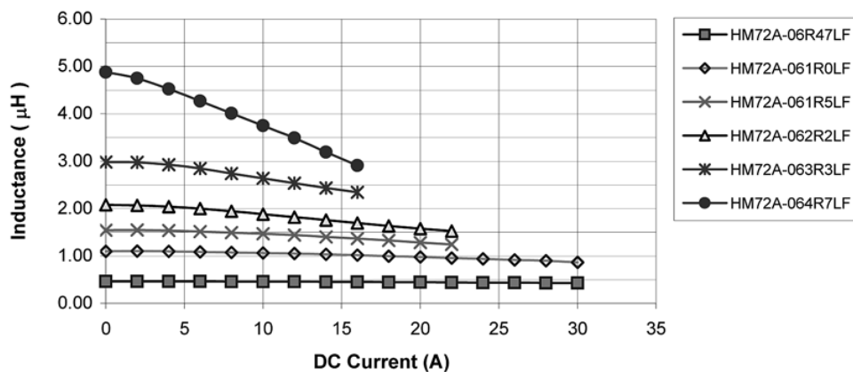
Inductance vs. Current Characteristics
