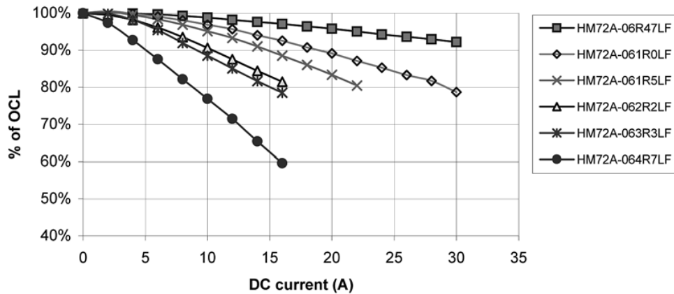
Inductance Rolloff vs. Current Characteristics
