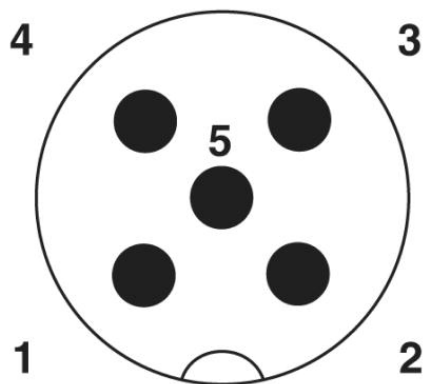
Pin assignment M12 male connector, 5-pin., A-coded, male side
