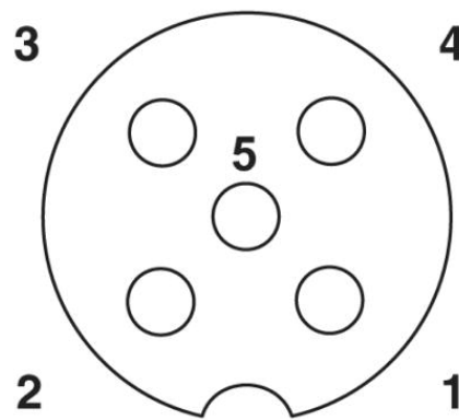
Pin assignment M12 socket, 5-pin., A-coded, socket side view
