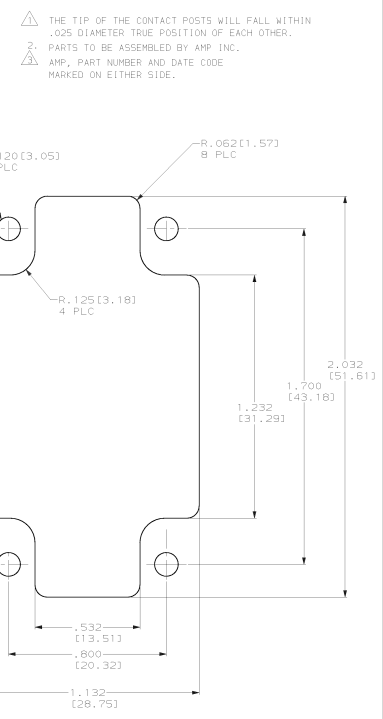
SUGGESTED PANEL CUTOUT SCALE 4:1
