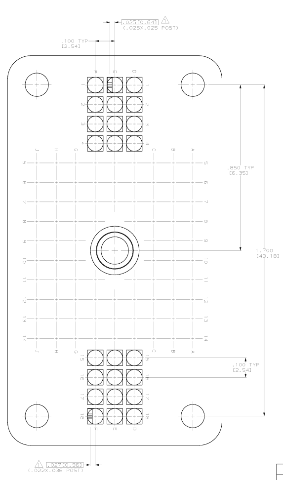
SUGGESTED PANEL CUTOUT SCALE 4:1
