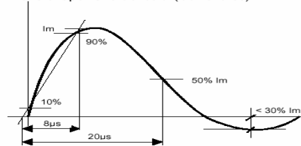
Wave shape "Short circuit" (Current I sc )
