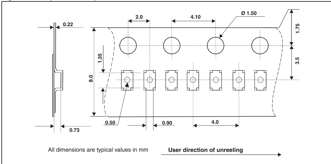
Figure 12. Tape and reel specification
