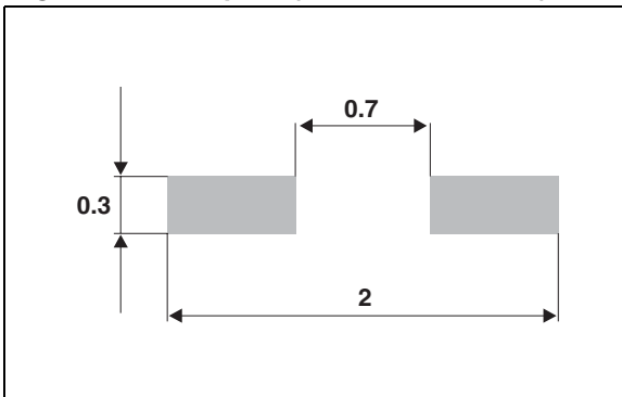
Figure 10. Footprint (dimensions in mm)
