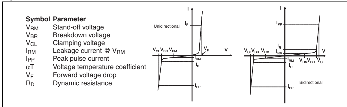
Figure 1. Electrical characteristics - definitions
