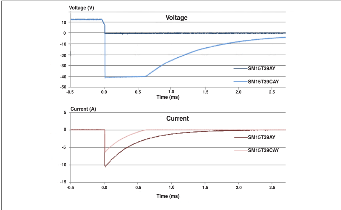
Figure 11. ISO7637-2 pulse 1 response ( V_S = -100\text{ V} )
