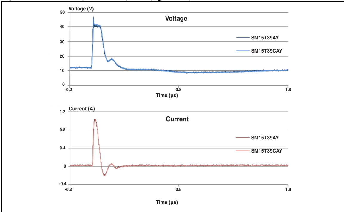
Figure 14. ISO7637-2 pulse 3b response ( V_S = 100\text{ V} )
