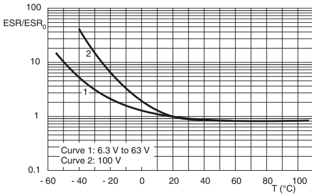
Fig.8 Typical multiplier of ESR as a function of temperature at 100 Hz ESR_0 = typical ESR at 20 °C, 100 Hz
