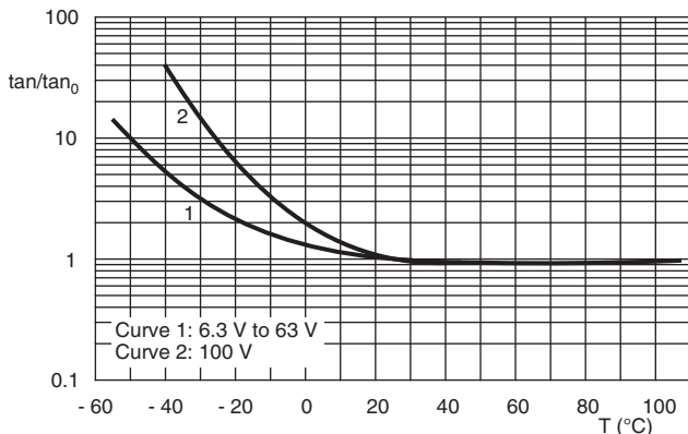
Fig.10 Typical multiplier of dissipation factor \tan \delta as a function of temperature at 20 °C at 100 Hz \tan \delta_0 = typical \tan \delta at 20 °C, 100 Hz
