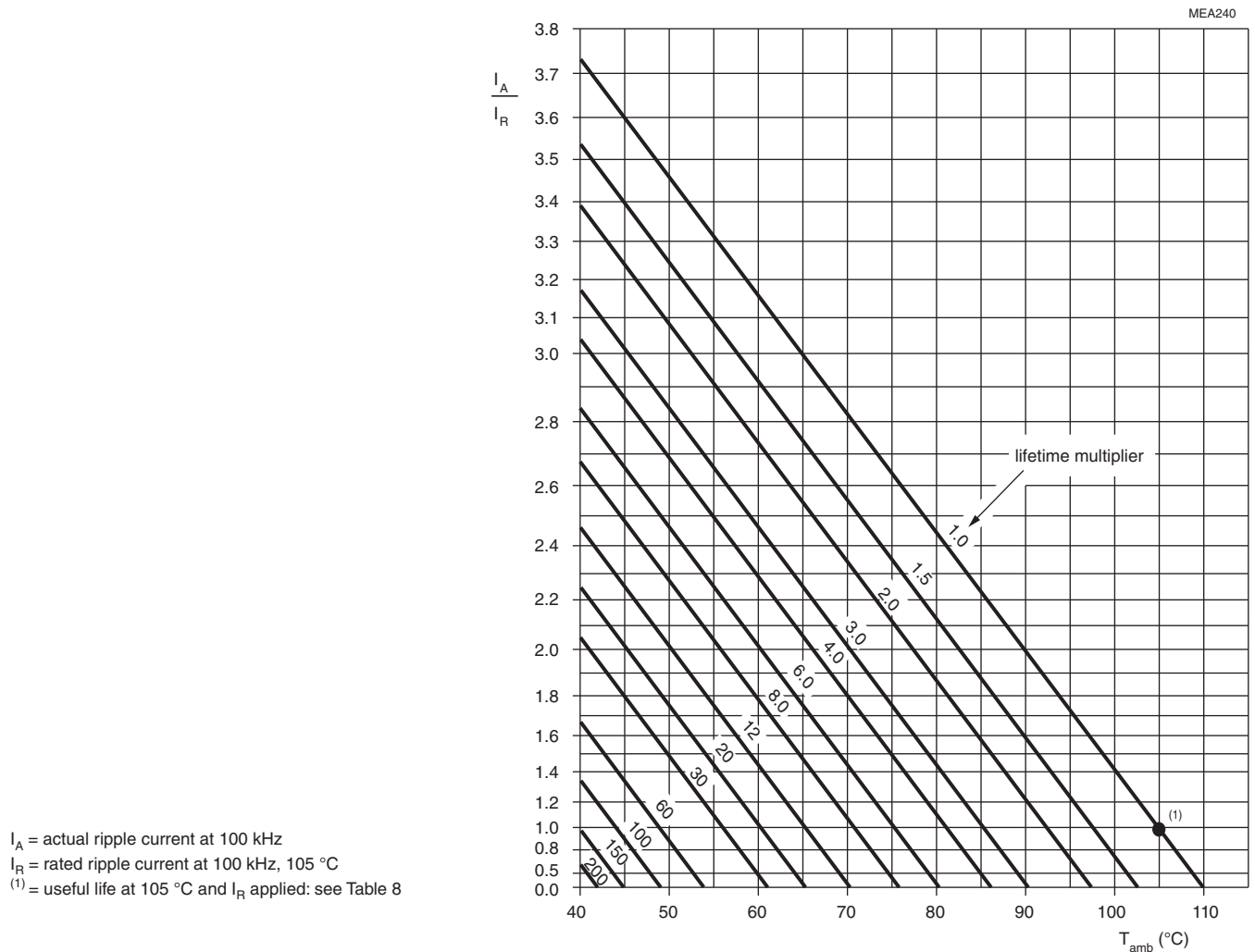
Fig.15 Multiplier of useful life as a function of ambient temperature and ripple current load
