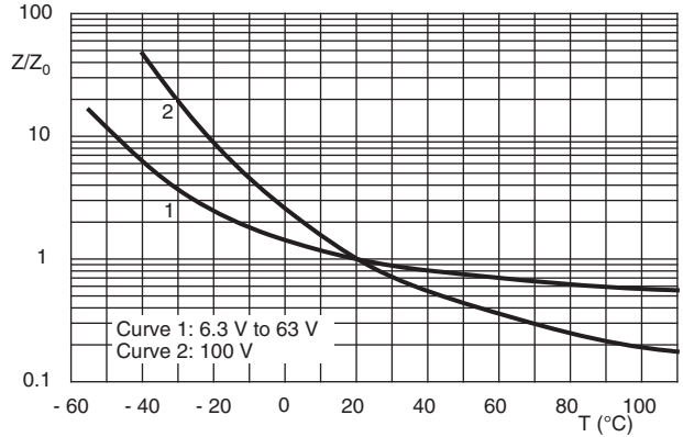
Fig.11 Typical multiplier of impedance Z as a function of temperature at 100 kHz Z_0 = typical impedance Z at 20 °C, 100 kHz
