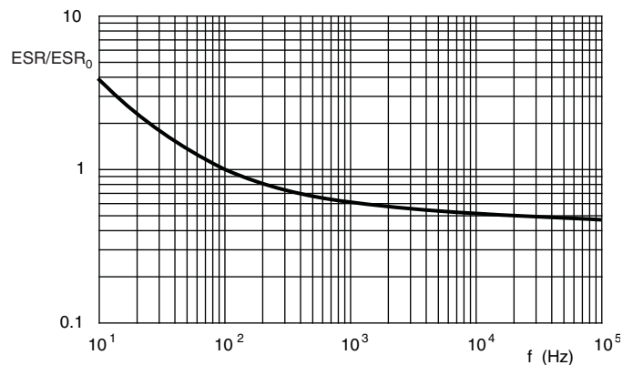
Fig.9 Typical multiplier ESR as a function of frequency at 20 °C ESR_0 = typical ESR at 20 °C, 100 Hz
