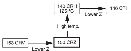
Fig.1 Component outline
