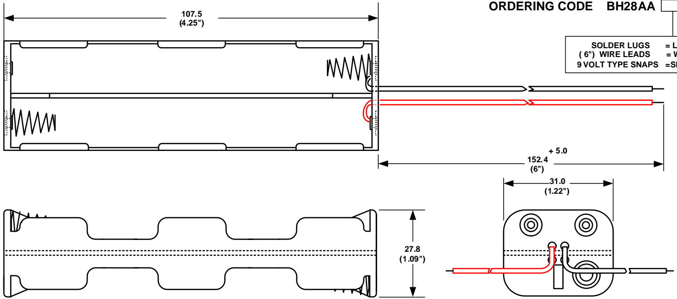
WIRE LEADS SHOWN ABOVE
