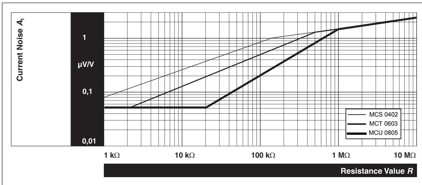
Fig.8 Current noise A 1 in accordance with IEC 60195.
