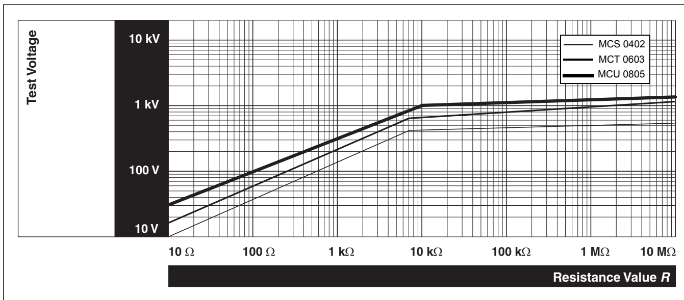
Fig.6 Pulse load rating in accordance with IEC 60115-1 clause 4.27; 1,2 μs / 50 μs; 5 pulses at 12 s interval; for permissible resistance change 0,5%.
