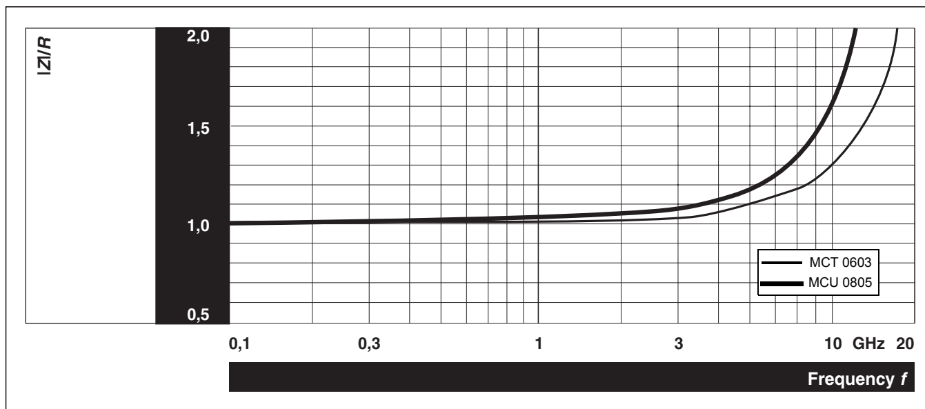
Fig.9 |Z|/R for 49,9 Ω chip resistor.
