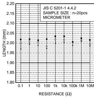
Fig.2 Dimensions (length)
