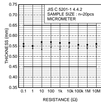
Fig.4 Dimensions (thickness)
