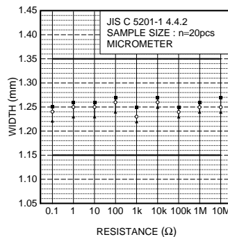
Fig.3 Dimensions (width)
