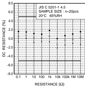
Fig.5 Resistance
