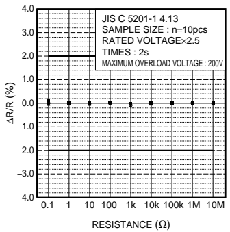
Fig.7 Overload
