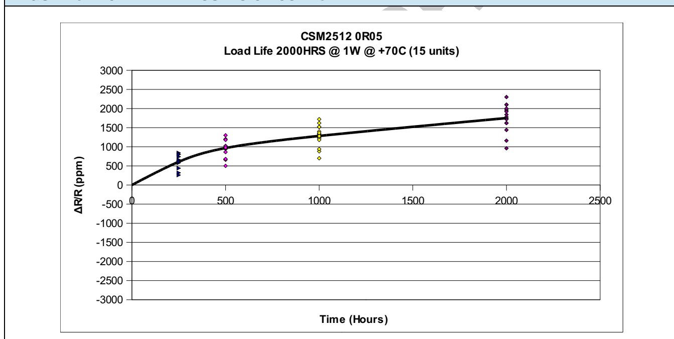
FIGURE 3 - LOAD LIFE RESULTS OF CSM2512
