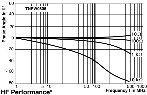
HF Performance*
