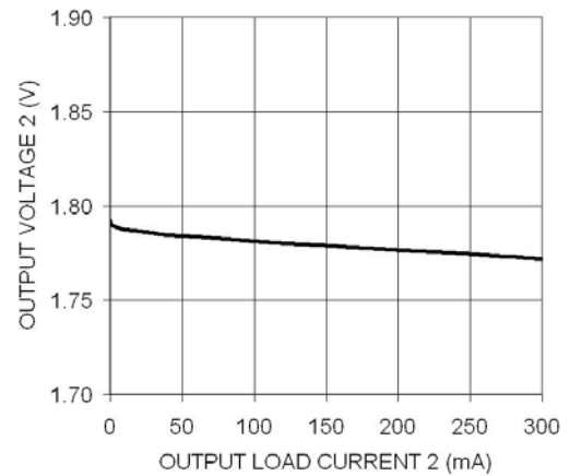
Figure 6. Load Regulation VOUT2
