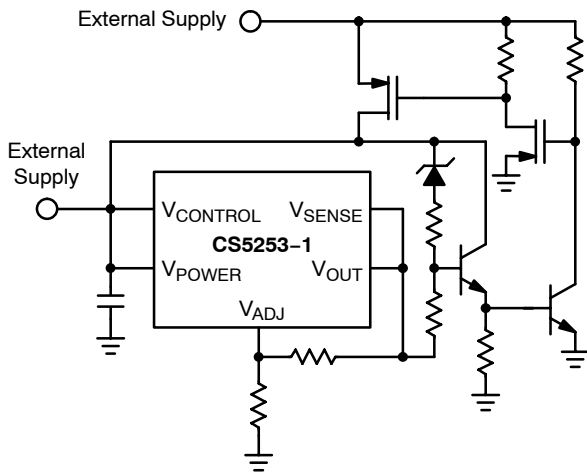
Figure 20. This Circuit Is an Example of How the CS5253-1 Can Be Short-Circuit Protected When Operating With V OUT > 6.0 V
