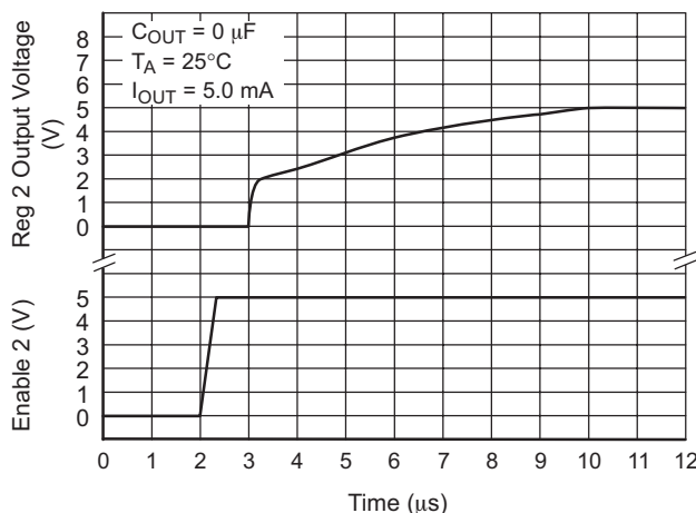
Figure 15. Regulator 2 Startup
